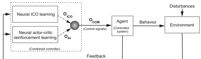
Fig. 1. Combinatorial learning framework with parallel combination of ICO learning and actor-critic reinforcement learning. Individual learning mechanisms adapt their weights independently and then their final weighted outputs ( O_{ico} and O_{ac} ) are combined into O_{com} using a reward modulated Hebbian plasticity rule (dotted arrows represent plastic synapses). O_{com} controls the agent behavior (policy) while sensory feedback from the agent is sent back to both the learning mechanisms in parallel.
