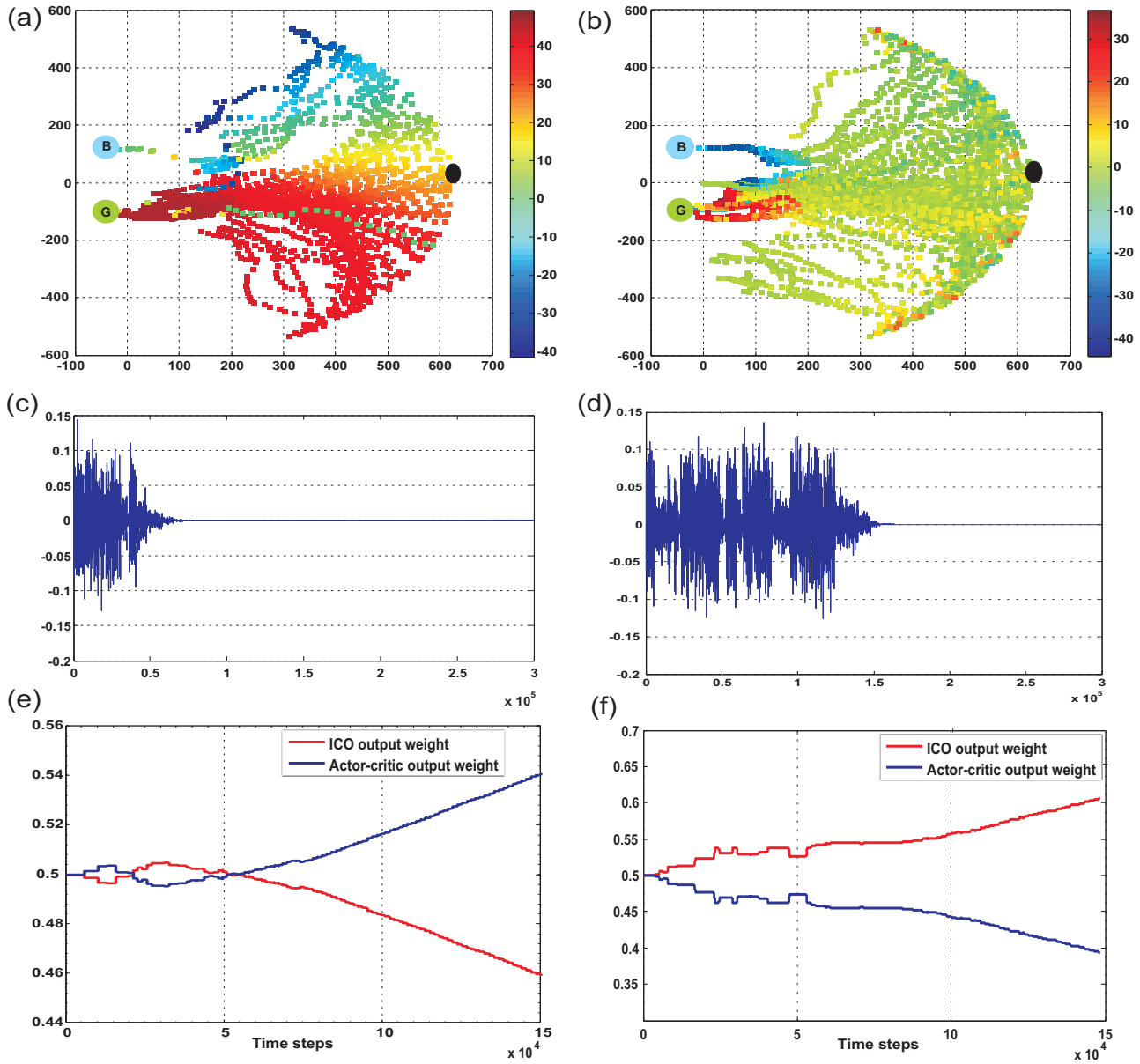
Fig. 5. (a) Estimation of the value function v(t) using reservoir based critic. The v(t) estimate is plotted with respect to local co-ordinates of the robot and an observer located directly opposite to the robot starting position. Colormap indicates the changing v(t) values. The black ball indicates the starting position of the robot with random orientation and the curvature of the plot is resultant of the shape of view from the observer. (b) Estimation of value function v(t) for the same task using the static RBF based critic. (c) Convergence of exploration term \epsilon(t) using reservoir critic. (d) Convergence of exploration term using RBF critic. (e) Adaptation of ICO weights \xi_{ico} and actor-critic weights \xi_{ac} using the RMHP rule for Combined learner with reservoir critic. (f) Adaptation of ICO weights \xi_{ico} and actor-critic weights \xi_{ac} using the RMHP rule for Combined learner with RBF critic. The continuous change in the learned weights even after successful learning of task is due to the Hebbian nature of the adaptation rule. This can be easily controlled by introducing additional synaptic scaling mechanism or in this case stop the weight updation once exploration ( \epsilon(t) ) becomes zero. All the plots were generated for the same goal-directed behavior task of reaching the green goal. The plots indicate the best performance case for each setup.
